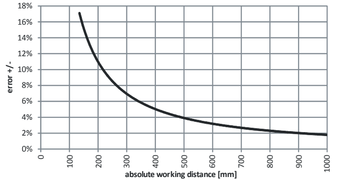
approx. intensity error for +/- 10mm distance change
